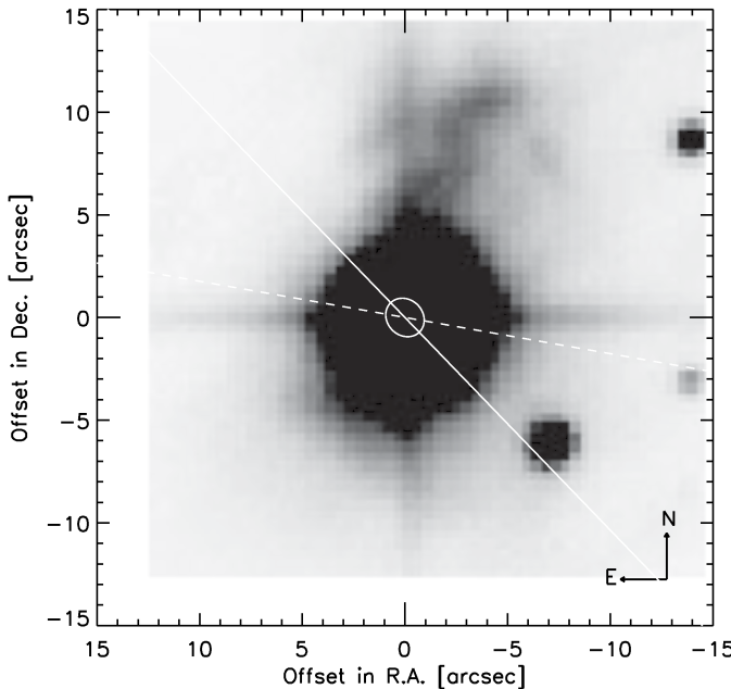
Fig. 8. K-band image of NGC 2264 IRS 1 from Schreyer et al. (1997). We overlay an ellipse (white) that shows a disk seen under an inclination of 30^\circ and a position angle of 40^\circ . The size of the disk is not drawn to scale. The solid white line shows the orientation of the 40 m baseline, the dashed one the orientation of the 90 m baseline.
