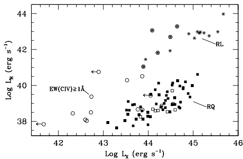
Fig. 1. The distribution of the PG quasars in the L_R vs. L_X plane. RLQs are designated by stars, and their L_R/L_X is on average a factor of 10^3 higher than for RQQs. Circles mark objects with C IV absorption EW > 1 \text{ \AA} (some of which are RL), where left attached arrows mark upper limits to L_X . These UV absorbed AGN tend to be underluminous by a factor of 10-30 in L_X for a given L_R due to absorption. Squares are RQQs without C IV absorption, where the filled/empty squares mark objects with radio detections/upper limits. Note the small scatter in the L_R vs. L_X correlation in RQQs, once RLQs and UV absorbed quasars are excluded.
