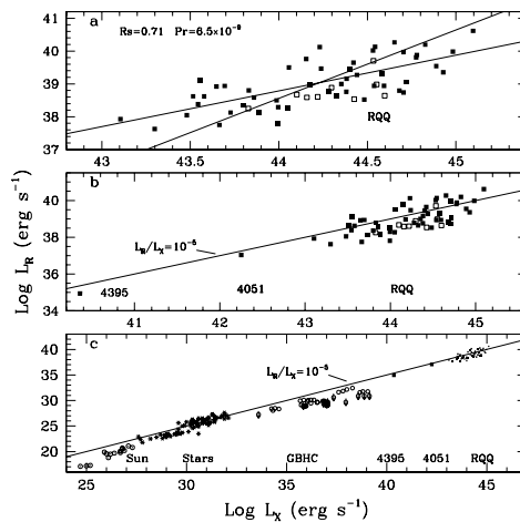
Fig. 2. Panel a, same as in Fig. 1, including only the RQQs without UV absorption. The Spearman rank order correlation strength and its significance is indicated in the upper left corner. The two lines mark least square fits minimizing the deviations in either L_R or L_X . Panel b, zoom out to include the two lowest luminosity type 1 AGN, which are well studied in the X-rays. Most objects are within a factor of few from the solid line which marks L_R/L_X = 10^{-5} (it is not a fit). Panel c, further zoom out to include GBHC, coronally active stars, and individual solar flares. Coronally active stars also lie close to L_R/L_X = 10^{-5} , which raises the possibility that both L_R and L_X in RQQs originate in coronal emission.
