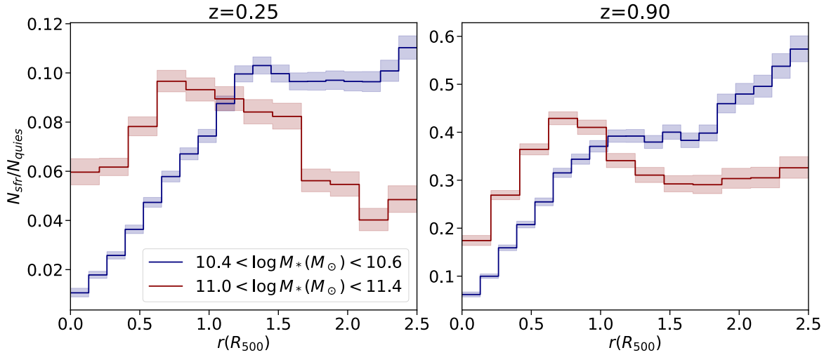
Figure 4.9: The ratio between the number of star-forming ( \text{SFR} > 0.02M_{\odot}/\text{yr} ) and quiescent galaxies as a function of clustercentric distance r , shown for two narrow M_* ranges (one in the massive and one in the low-mass range). Profiles are shown at low redshift (left panel) and high redshift (right panel). The profiles are qualitatively similar to those in figure 4.8, where a wider M_* range was used.
