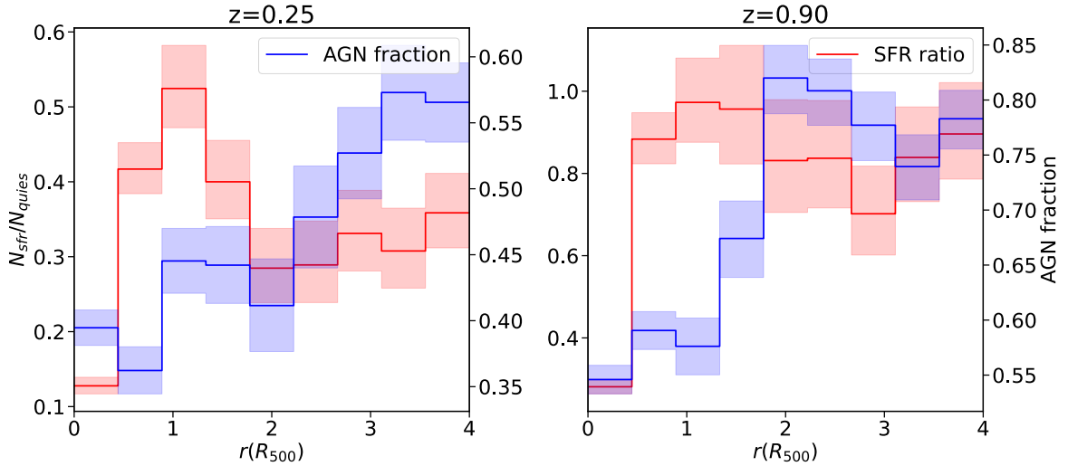
Figure 5.14: The AGN fraction of massive galaxies with constant local density ( 1.8 < \log d_n(\text{kpc}) < 1.9 ), and the ratio between massive star-forming and massive quiescent galaxies. The figure can be compared with figure 5.5, where no d_n selection is made.
