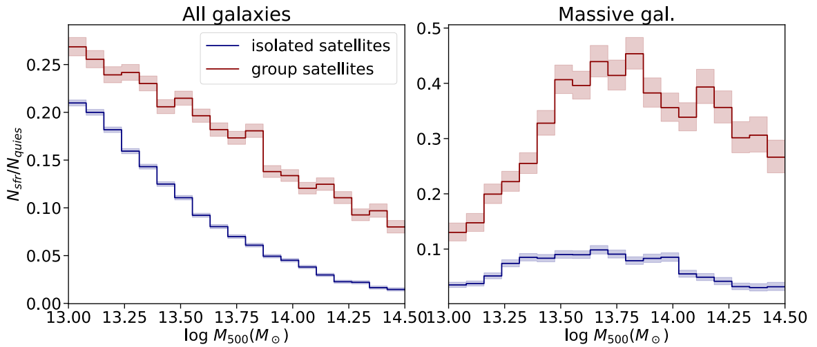
Figure 4.15: The ratio between the number of star-forming ( \text{SFR} > 0.02M_{\odot}/\text{yr} ) and quiescent galaxies as a function of the cluster mass M_{500} , shown for group satellites and isolated satellites (see section 4). The ratio for all galaxies (mostly low-mass galaxies) is plotted on the left panel, and the ratio for massive galaxies is shown on the right panel. Results are shown at low redshift ( z = 0.25 ). The BCGs are excluded.
