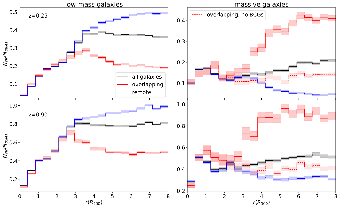
Figure 4.7: The ratio between the number of star-forming ( \text{SFR} > 0.02M_{\odot}/\text{yr} ) and quiescent galaxies as a function of clustercentric distance r . On the left, I show low-mass galaxies with 10.15 < \log M_*(M_{\odot}) < 11 , and on the right only massive galaxies with \log M_*(M_{\odot}) > 11 . Results are shown at low redshift (upper panels) and high redshift (bottom panels) and for the overlapping and remote regions (with overlapping distance 6R_{500} , refer to chapter 3). On the right panels, the dashed line represents the massive overlapping populations without the BCGs of the neighbouring groups with M_{500} > 10^{13}M_{\odot} . Errors are derived from Poisson statistics (see appendix A.1).
