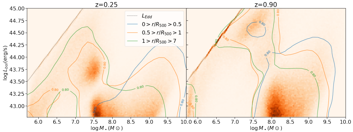
Figure 5.1: Distribution of black hole masses M_{\bullet} and their bolometric luminosities at low redshift (left panel) and high redshift (right panel). Contours represent the 80% confidence intervals of the black hole parameter distributions in different radial shells around the clusters (radial range is shown in the legend). The 2D color histogram represents the distribution of all galaxies in the extended cluster regions (from 0 to 7 R_{500} ). The dotted line, traced by an excess of AGNs on the top left of each panel, represents the bolometric luminosity of black holes accreting with Eddington mass accretion rate (equation 2.2). The minimal bolometric luminosity shown ( 5.9 \cdot 10^{42} erg/s) corresponds to 10^{42} erg/s in 0.5-10 keV band, which is mostly used as the AGN selection threshold in this chapter.
