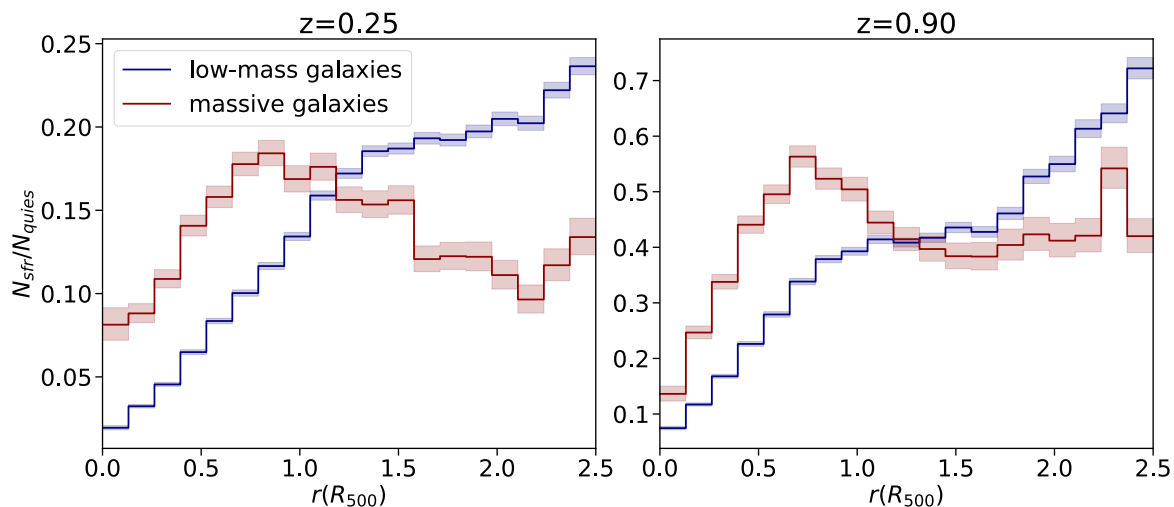
Figure 4.8: The ratio between the number of star-forming ( \text{SFR} > 0.02M_{\odot}/\text{yr} ) and quiescent galaxies as a function of clustercentric distance r shown for low-mass and massive galaxies at high redshift (right panel) and low redshift (left panel) in the inner cluster regions . Plots represent the zoomed-in versions of the combined plots in figure 4.7.
