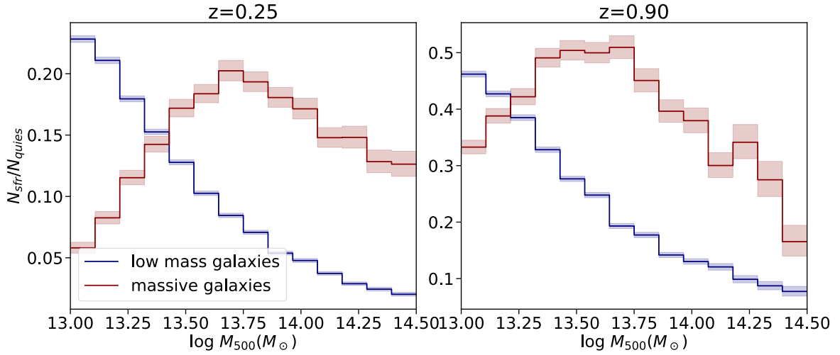
Figure 4.14: The ratio between the number of star-forming ( \text{SFR} > 0.02M_{\odot}/\text{yr} ) and quiescent galaxies as a function of the cluster mass M_{500} for low-mass and massive galaxies at high redshift (right panel) and low redshift (left panel). Regions up to 2R_{500} are considered. The BCGs are excluded.
