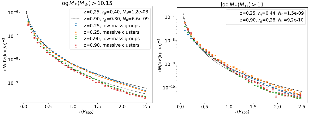
Figure B.2: Radial distribution of galaxies in low-mass ( 13 < \log M_{500}(M_{\odot}) < 14 ) and massive clusters ( \log M_{500}(M_{\odot}) > 14 ) at low and high redshift. Combined data of low-mass groups and massive clusters (between 0.05 and 2R_{500} ) were used for fitting. On the left panel, all galaxies were used, while on the right panel, only massive galaxies were selected.
