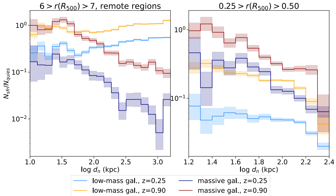
Figure 4.12: The ratio between the number of star-forming ( \text{SFR} > 0.02M_{\odot}/\text{yr} ) and quiescent galaxies as a function of the distance to the nearest neighbour d_n . Results are shown for low and high redshift and for low-mass and massive galaxies. On the left panels, isolated regions between 6R_{500} and 7R_{500} are selected, and on the right panel, I choose the cluster regions between 0.25 and 0.5R_{500} ; narrow radial bins are chosen to distinguish the effects of the local density from the effects of the global cluster environment. Errors are derived in A.1.
