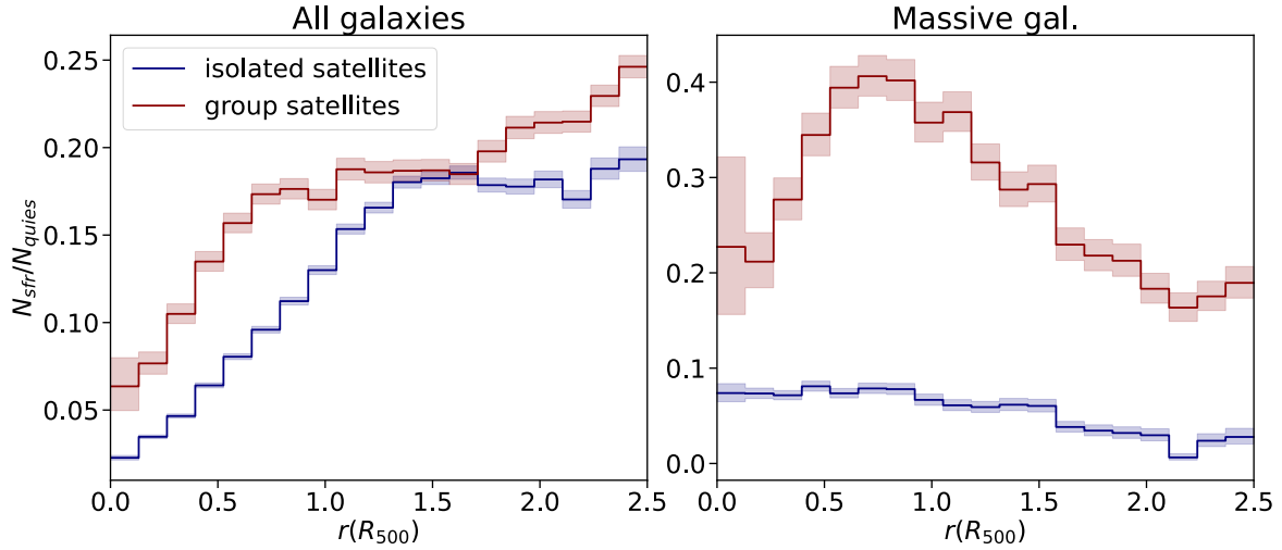
Figure 4.10: The ratio between the number of star-forming ( \text{SFR} > 0.02M_{\odot}/\text{yr} ) and quiescent galaxies as a function of clustercentric distance r , for galaxies that belong to groups with multiple galaxies embedded into the central cluster halo (i.e., group satellites), and for galaxies which belong to directly to the central cluster halo (i.e., isolated satellites, see section 4). The ratio for all galaxies (mostly low-mass galaxies) is plotted on the left panel, and the ratio for massive galaxies is plotted on the right panel. The profiles are shown at low redshift ( z = 0.25 ).
