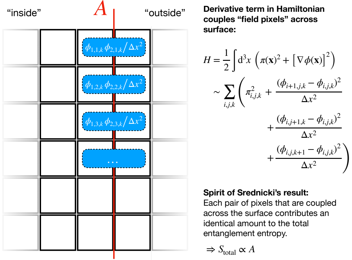
Figure 9: Sketching how short-range coupling of field modes across a surface A lead to an area scaling of the entanglement entropy across that surface.
