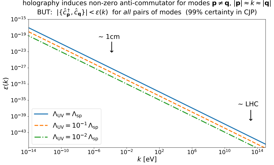
Figure 17: Figure from [51], showing their bound on the anti-commutator \{\hat{c}_{\mathbf{p}}^\dagger, \hat{c}_{\mathbf{q}}\} induced for modes \mathbf{p} \neq \mathbf{q} , |\mathbf{p}| \approx k \approx |\mathbf{q}| , due to squeezing the Fourier modes of a Weyl field into a Hilbert space whose dimension satisfies an area scaling (as opposed to the volume scaling of usual quantum field theory).
