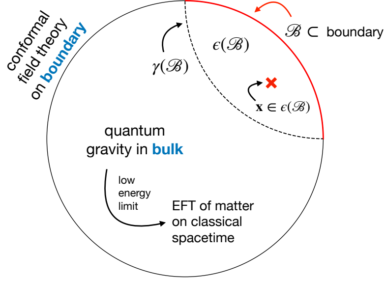
Figure 13: Sketch of the AdS/CFT correspondence
