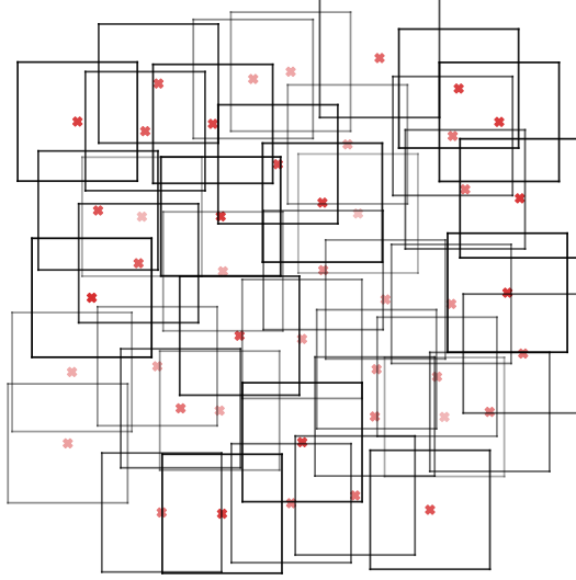
Figure 16: Figure from [51]: The Weyl field can be decomposed into a collection of qubits, which are represented by points \mathbf{p} in Fourier space (upper sketch). In 3 dimensions, the number of qubits in a small Fourier space shell s (red crossed in upper sketch) scales as k_s^2 \Delta_s where k_s is the radius and \Delta_s is the width of the shell. We want to embed these qubits into a Hilbert space that is strictly smaller than the tensor product of the individual qubit Hilbert spaces in order to achieve a holographic scaling of the effective degrees of freedom in our field.
