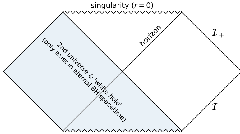
Figure 19: Penrose diagram for the Schwarzschild blackhole
