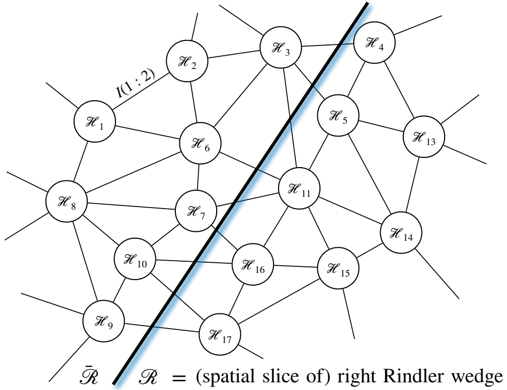
Figure 12: Same as Figure 11, but with the region \mathcal{R} now representing a constant-time slice of a Rindler wedge of the emergent spacetime.
