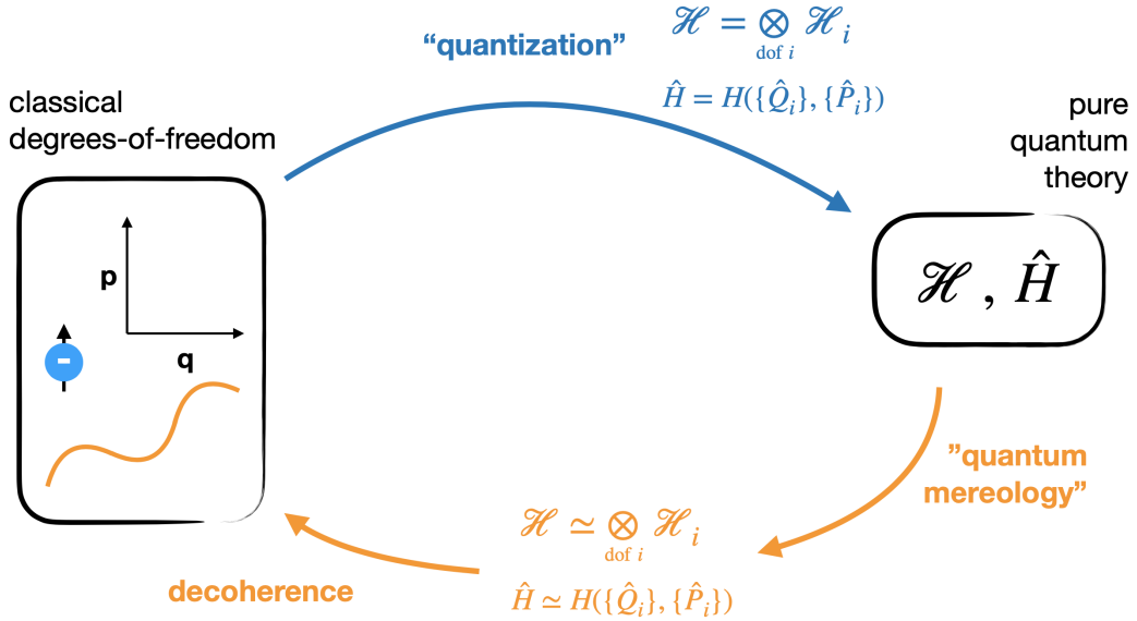
Figure 10: The process of quantisation turns a classical theory into a quantum theory. Quantum mereology (+ decoherence) on the other hand, tries to identify classical dynamics in a Hamiltonian that was defined without any reference to quantised classical variables (e.g. just a random matrix).
