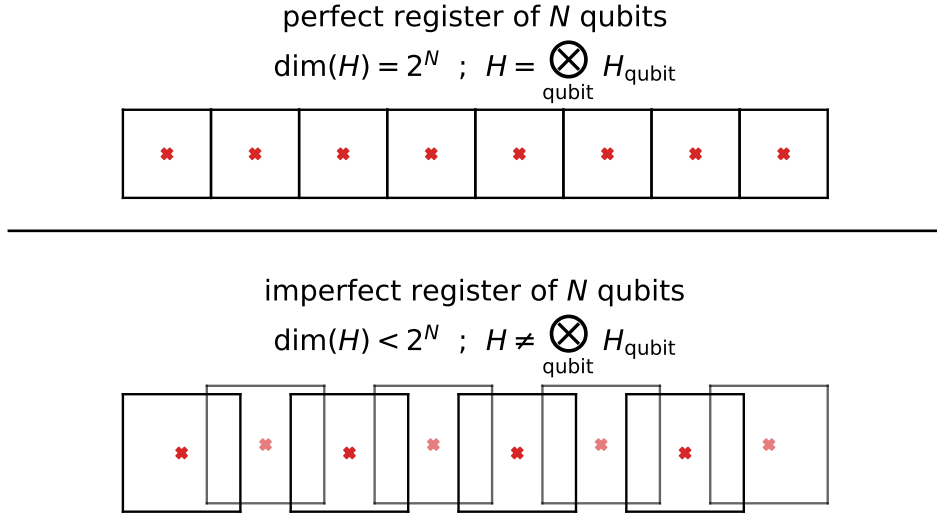
Figure 15: Figure from [51]: The upper sketch illustrates a perfect qubyte consisting of eight non-overlapping qubits. The Hilbert space of the entire qubyte is the tensor product of the individual qubit Hilbert spaces. The lower sketch illustrates the situation when the total Hilbert space is strictly smaller than such a tensor product. In this case the qubits must be overlapping, i.e. the Pauli algebras that define the different qubits are not (anti-)commuting.
