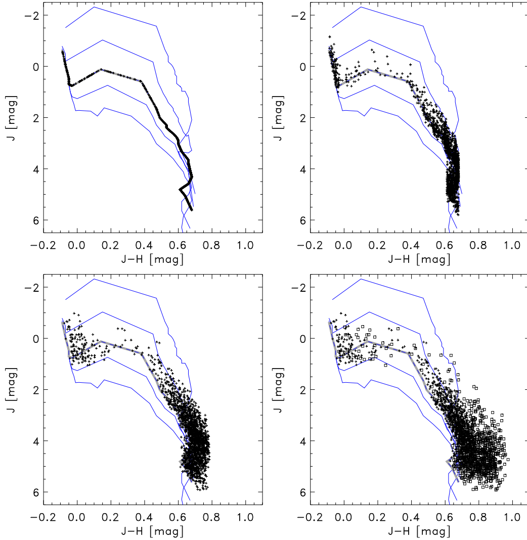
Fig. 4 Different stages of the Monte-Carlo simulation of a Near-Infrared Color-magnitude diagram for a perfectly co-eval cluster of 6000 stars with identical ages of 3 Myr and a distribution of masses between 0.1 M_{\odot} and 7 M_{\odot} according to the Kroupa (2002) IMF. The blue lines show the isochrones for ages of 0.1 Myr, 1 Myr, 3 Myr, 5 Myr, and 10 Myr according to the Siess et al. (2000) models. The “true” isochrone for 3 Myr is emphasized by the thick gray line. The crosses show the positions of the simulated stars. The upper left panel shows the theoretically expected magnitudes of the simulated stars. In the upper right panel, the effects of unresolved binaries and the stellar variability (as described in Sect. 3) is included. In the lower left panel, the effect of differential extinction (following a uniform distribution in the range A_V = [0 - 1] mag) is added. In the lower right panel I added infrared excess emission to 20% of the stars (marked by open boxes), assuming a uniform distribution of \Delta(J - H) values in the [0 - 0.2] mag range according to Meyer et al. (1997).
