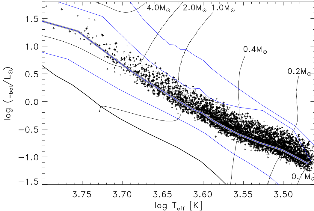
Fig. 2 Monte-Carlo simulation of a HRD for a perfectly co-eval model cluster of 6000 stars with identical ages of 3 Myr and a distribution of masses between 0.1 M_{\odot} and 7 M_{\odot} according to the Kroupa (2002) IMF. The black lines show evolutionary tracks for different stellar masses according to the Siess et al. (2000) models. The blue lines show the isochrones for ages of 0.3 Myr, 1 Myr, 3 Myr, and 10 Myr, and the ZAMS (thick black line). The pluses show the positions of the stars after including the simulated observational uncertainties described in the text, while the thick gray line marks the theoretical 3 Myr isochrone.
